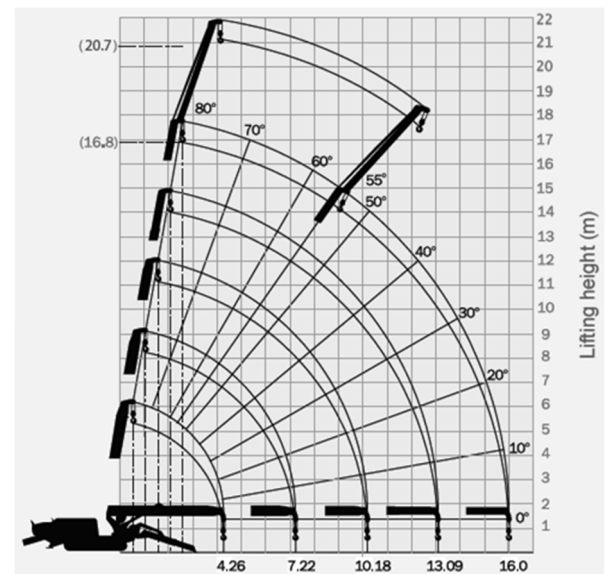
Working radius (m)
